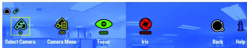
Figure 16. Cameras Menu
